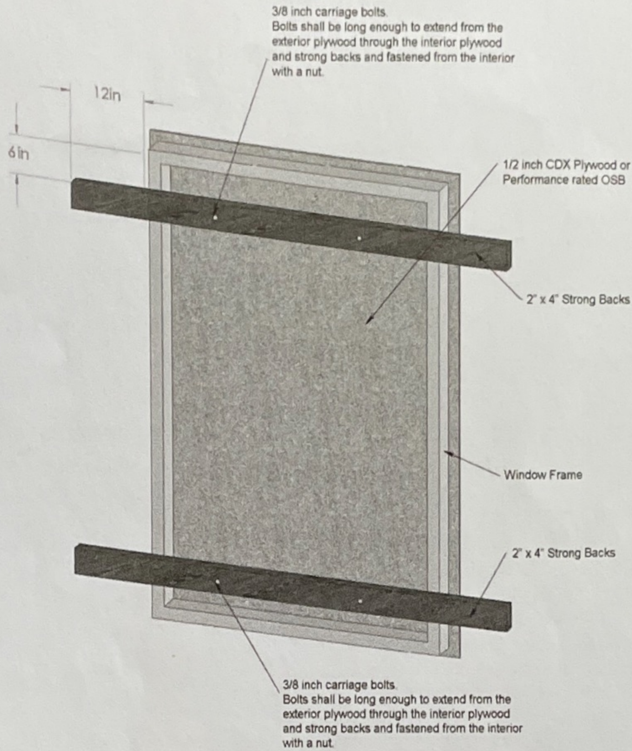
FIGURE A103.1(1) BOARDING OF DOOR OR WINDOW
