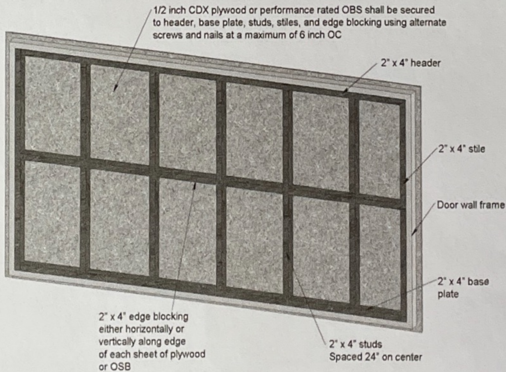
FIGURE A103.1(2) BOARDING OF DOOR WALL
